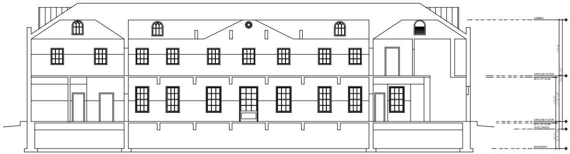
1 EXISTING SECTION LOOKING SOUTH SCALE: 1/8" = 1'-0"
